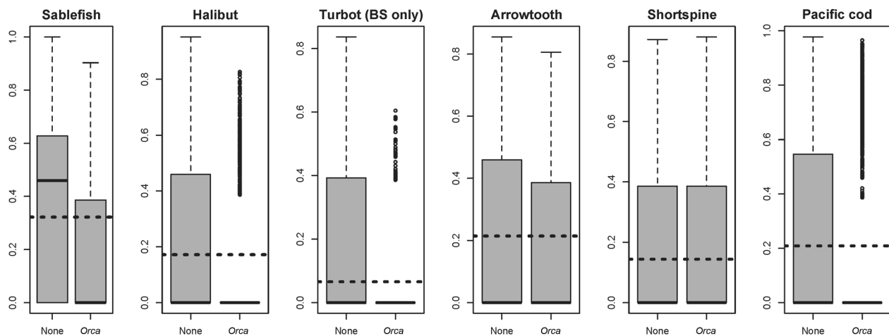
Figure 3. Groundfish cpue averaged over time and across all survey stations, with (“Orca”) and without (“None”) killer whales present, NMFS longline survey 1998–2011. Black bars denote median, dotted lines denote overall mean, grey boxes denote lower and upper quartiles, and whiskers extend to the closest observation that is < 1.5 times the interquartile range from the upper quartile.
